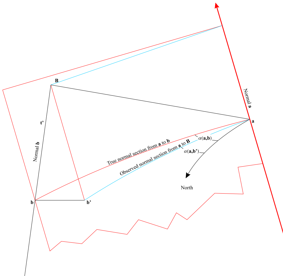
FIGURE 19. The observing station is on the normal at a and the target station is at B . When B is not on the ellipsoid, the observed azimuth from a to B varies from the true value to do the normal at b being skew to the normal at a .
