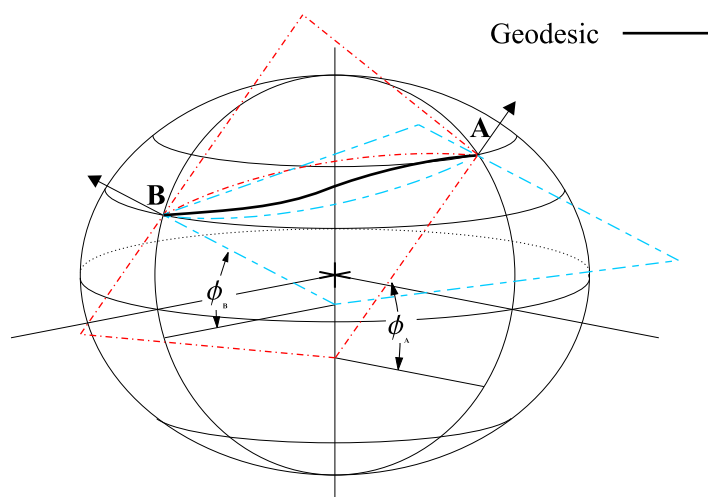
FIGURE 18. A composite picture putting Figure 15 with Figure 17. Note how the normal vectors intersect the z-axis in different locations, and that they are not coplanar. The geodesic from A to B is shown between the normal sections as a bold solid curve.
