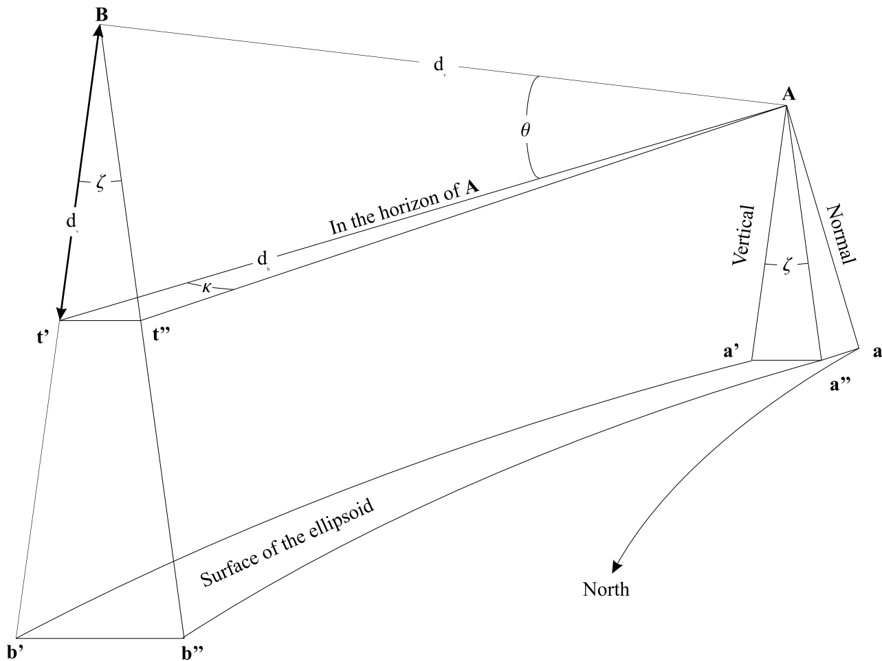
FIGURE 16. The deflection of the vertical.
