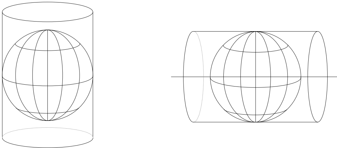
FIGURE 9. Two cylindrical projections. On the left is a standard cylindrical projection. The axis of the standard cylindrical projection is coincident with the minor axis. On the right is a transverse cylindrical projection. The axis of the transverse cylindrical projection is in the Equatorial plane.
