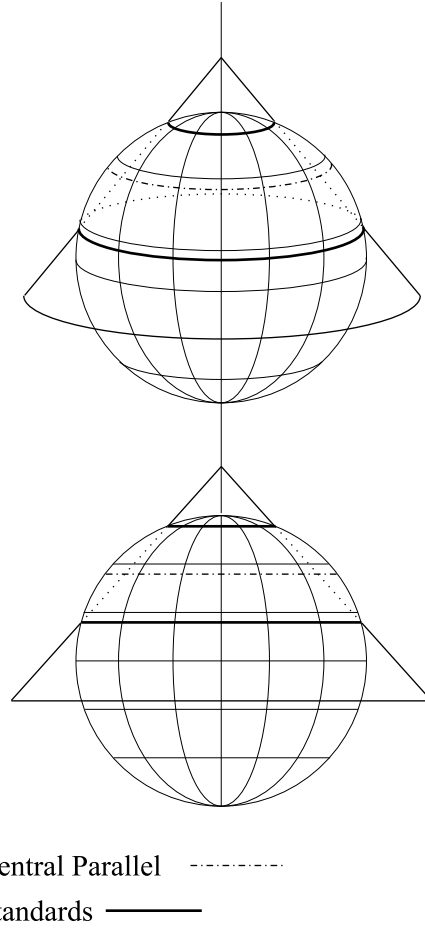
FIGURE 11. A conic projection with two standards. The standards are the heavier lines north and south of the central parallel. Note that the standards are also parallels.
